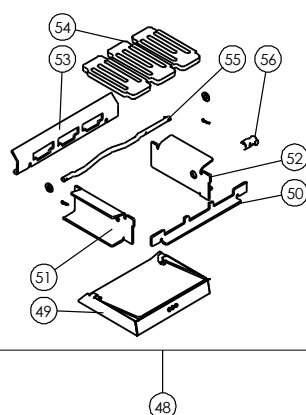
Optional Wood Ash Removal Kit
